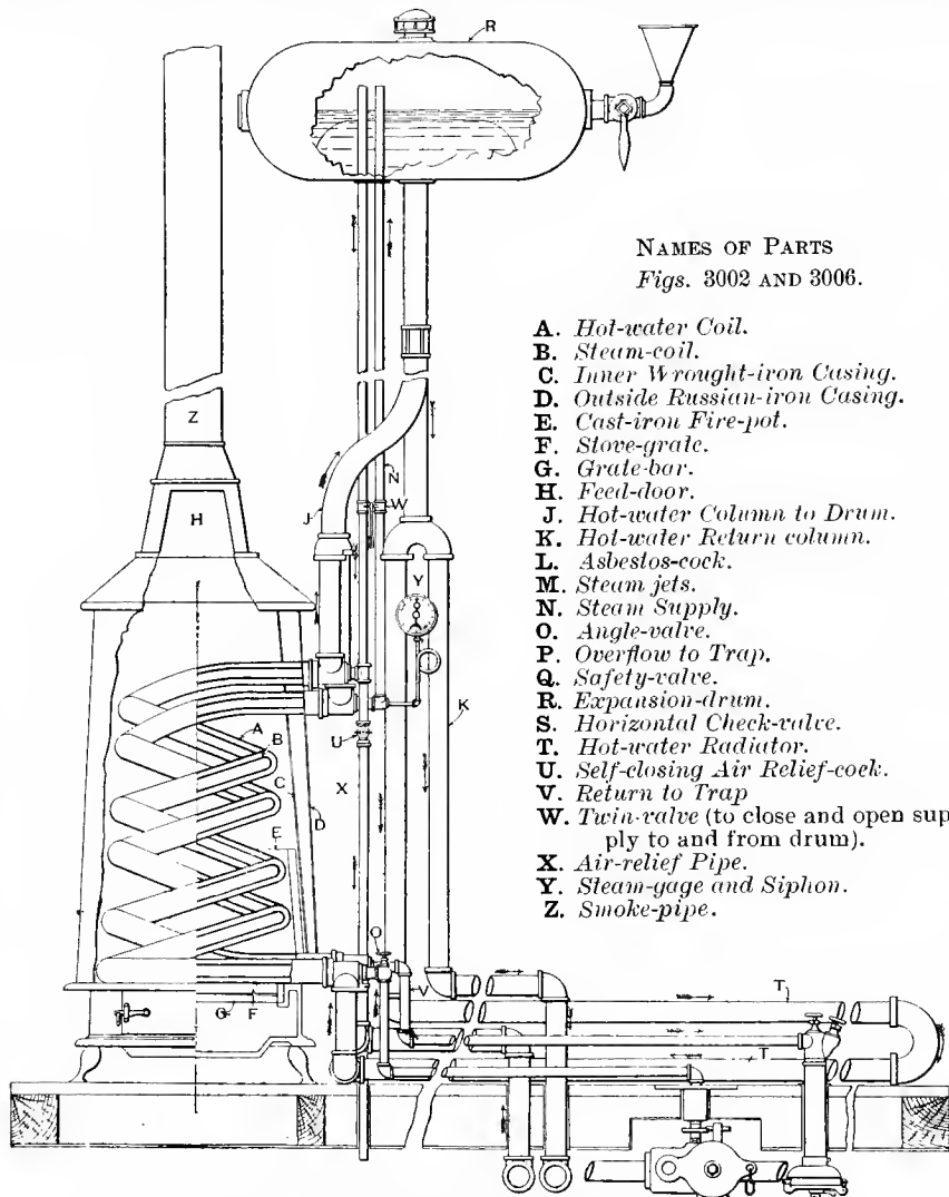
Fig. 3002. Sectional View of Heater and Pipe Connections. DUPLIX DOUBLE-COIL OVERFLOW SYSTEM.
